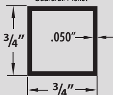
Guardrail Picket
